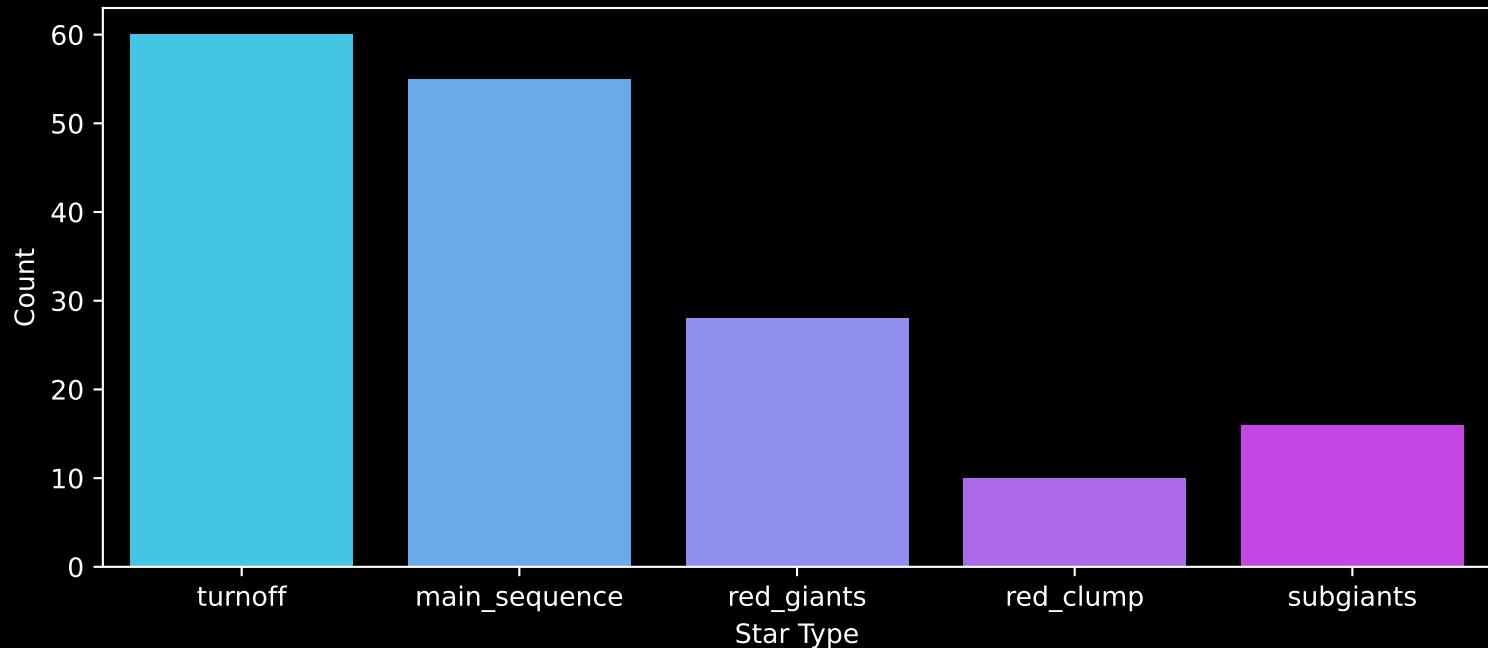
GALAH DR4 Field: [7142] Count plot of Star Type
